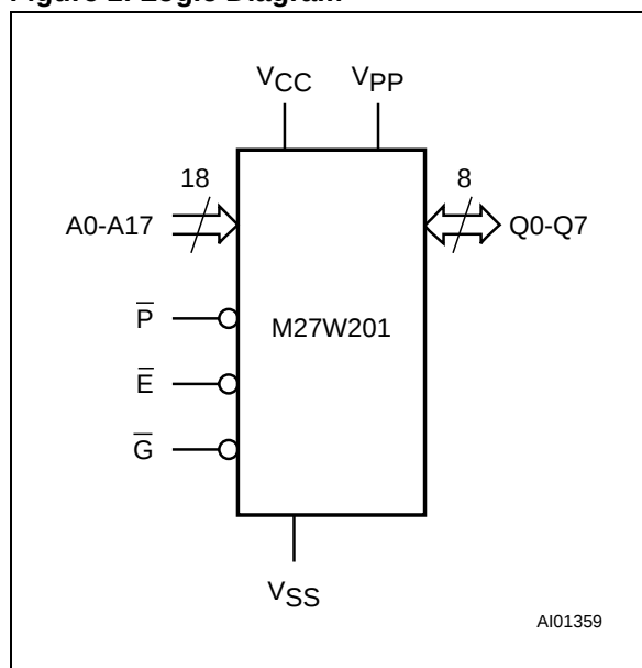
Figure 1. Logic Diagram
